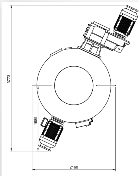
Illustrations: Dimensions of the Glomix-Glaxiaris® 3800 mixer with a gross volume of 3800 l and a useful volume of 80-90 %.
