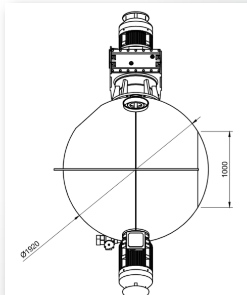
Illustrations: Dimensions of the Glomix-Glaxiaris® 3800 mixer with a gross volume of 3800 l and a useful volume of 80-90 %.
